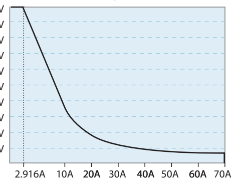
Model 63323A Input Characteristics
